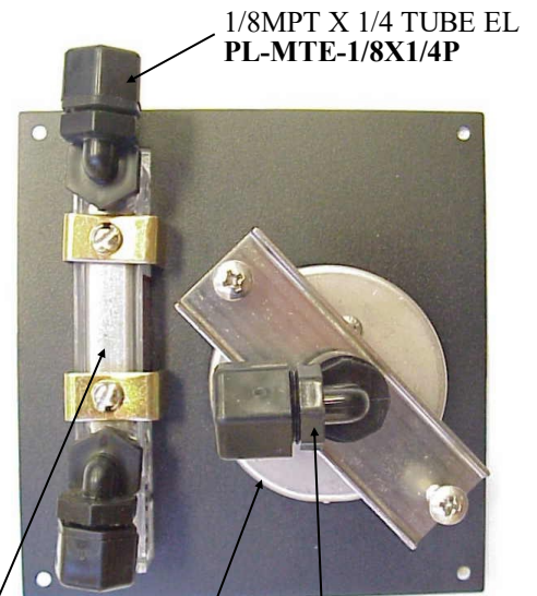
Pressure Gauge PL-PSG-LP2.5
