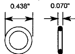
O-ring (8013008) Qty: 1
