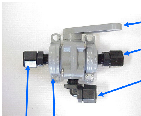
1/4" 3-Way Valve PL-VLV-3W1/4
