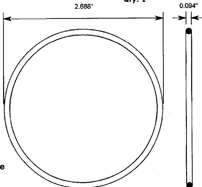
O-ring (8012830) Qty: 2
